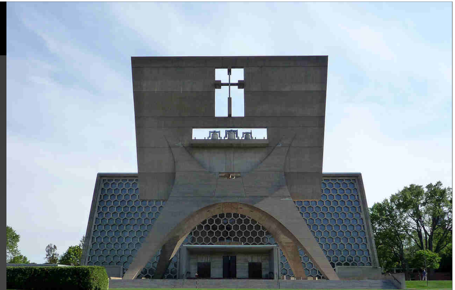
Marcel Breuer, Saint-John Abbey, 1953-1961, Collegeville, Minnesota
