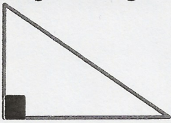
triangle rectangle
